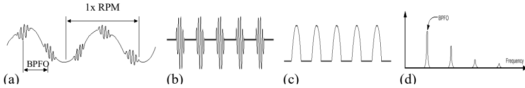
Fig. 1 : Envelope detection process (a) Unfiltered Time Signal (b) Bandpassed Time Signal (c) Envelope of Bandpassed Signal (d) Envelope Spectrum
